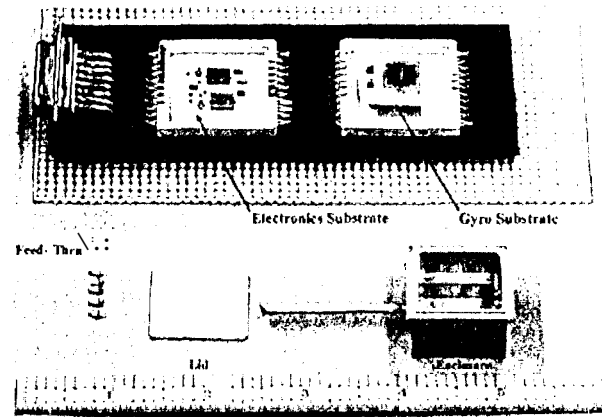
Figure 9. The components of the microgyroscope package.
