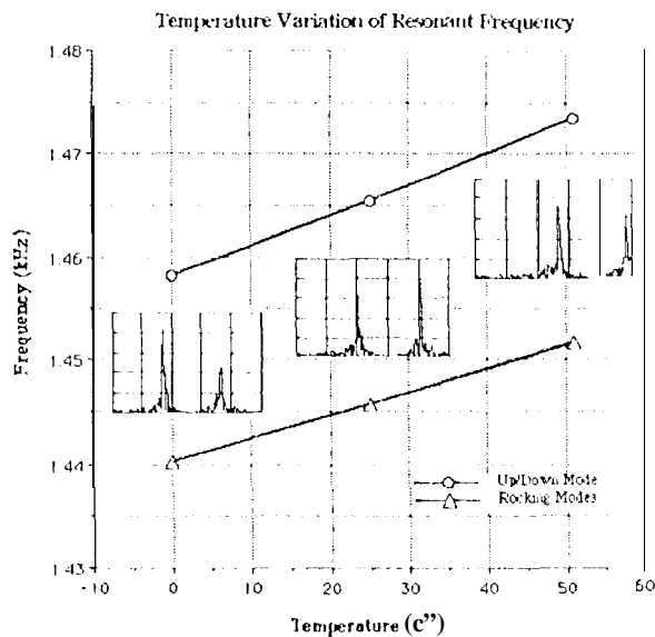
Figure 14. Temperature dependence of resonant frequency of the silicon clover-leaf structure.
