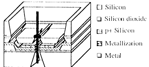
Figure 4. Cross-sectional view of the complete microgyroscope.
