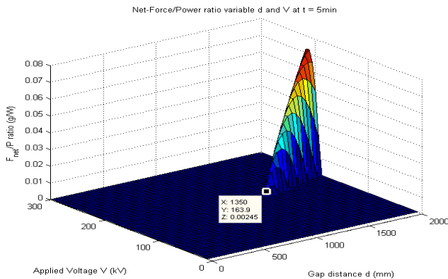
Fig. 9. Net-Force/Power ratio with variable gap distances and applied voltages for t = 5 min ( K_e = 0.001755 mA/mm \cdot kV ^2 , K_f = 0.005238 g/mm ^{0.46} .kV ^2 , R_b=6.1 g/W \cdot h, R_t=0.864 g/W).
