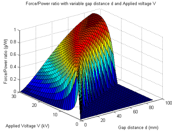
Fig. 3. Variation of Force-to-Power ratio with gap distance and applied voltage. ( K_e = 0.001755 \text{ mA/mm} \cdot \text{kV}^2 , K_f = 0.005238 \text{ g/mm}^{0.46} \cdot \text{kV}^2 ).
