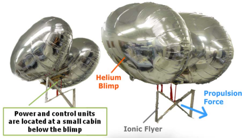
Fig. 11. Prototype of the Ionic Propulsion Blimp.
