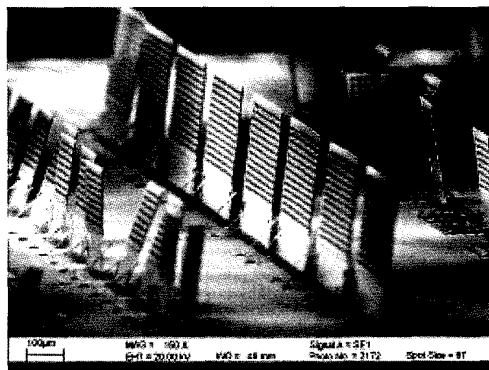
Figure 6. The batch micro-assembled mirror arrays.
