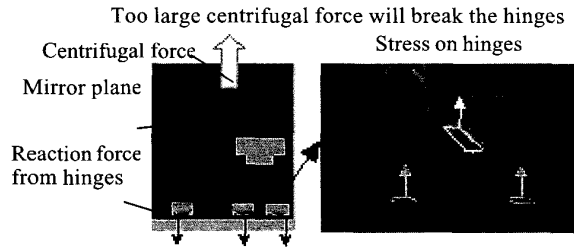
Figure 2. Stress acting on the polysilicon.
