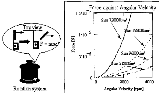
Figure 1. Conceptual drawing for centrifugal force applied on micro mirrors. Theoretically, centrifugal force can be generated on different sizes of MUMPs structures (poly1, poly2, and gold) by changing the angular velocity of a spinning disc.
