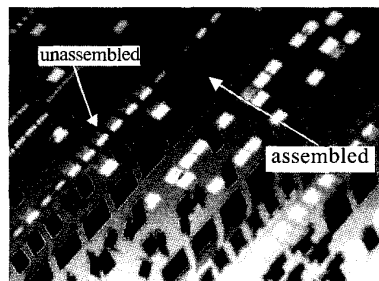
Figure 4. Different sizes of mass assembled by centrifugal force. The white structures in the picture represent the unassembled structures (reflection from gold layer), and the gray structures are the assembled structures with black shadows.
